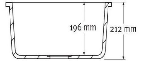
FRONT CROSS-SECTION
