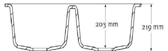
FRONT CROSS-SECTION
