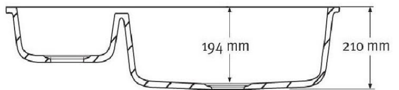
FRONT CROSS-SECTION
